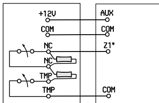
Czujka (2EOL/NC) PRIMA64/EXT-Z8
